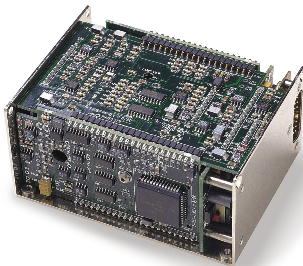
Assembled PRS10
