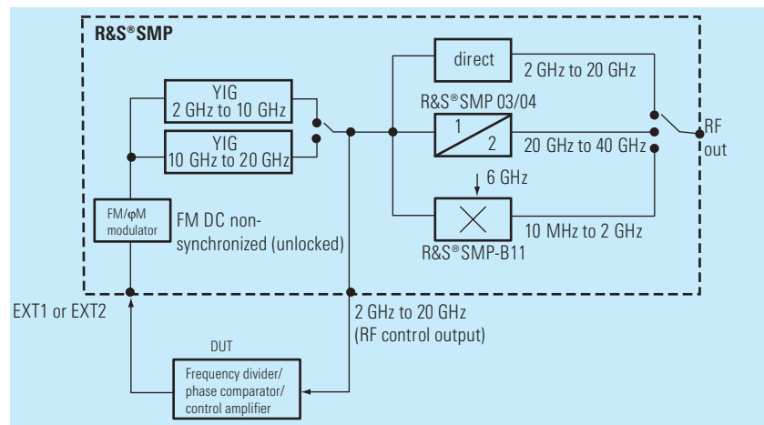
FIG 3: R&S®SMP as a VCO
