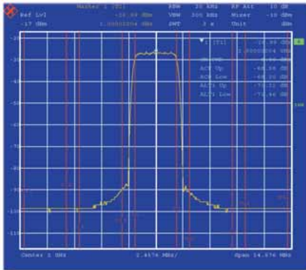
ACPR measurement for a WCDMA signal with option R&S SMIQB47
