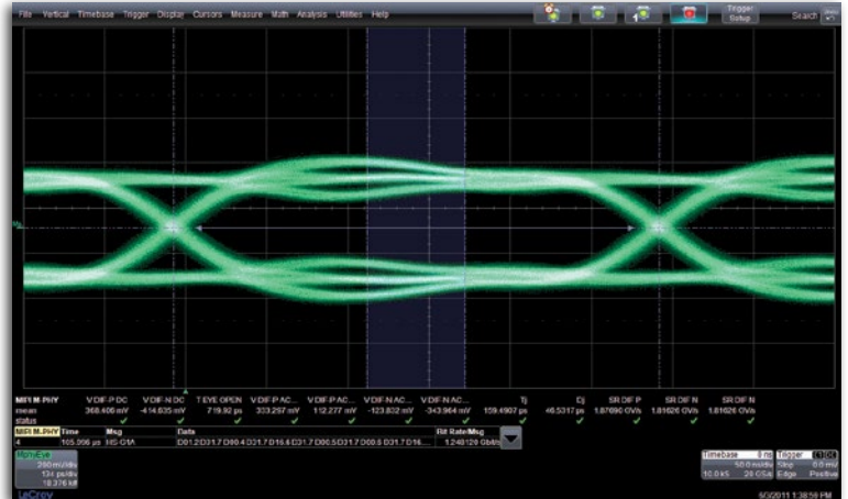
The eye diagram of an M-PHY signal illustrates portions of the eye that pertain to a specific measurement.
