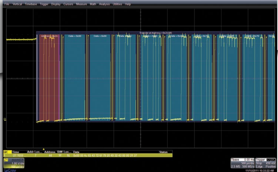
Color-coded overlaid protocol decode makes it easy to understand your serial data messages.
