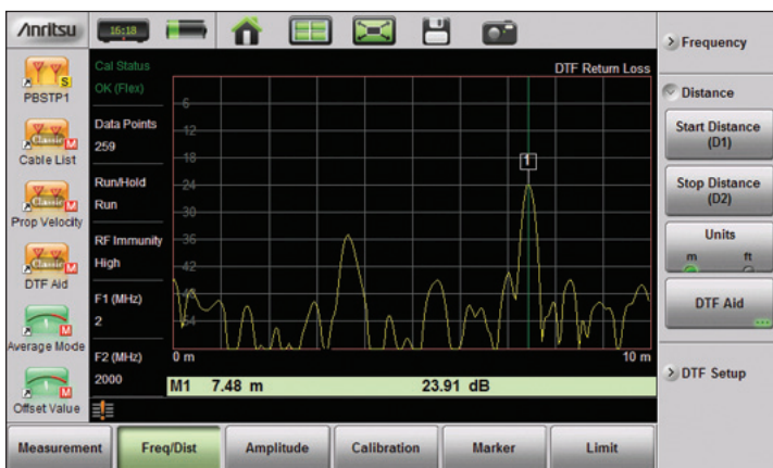
Distance-to-Fault measurement screen (Advanced Mode)
