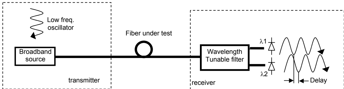
Figure 7: Differential phase-shift principle
