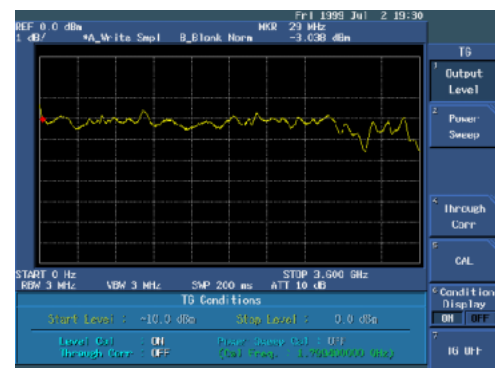
< Tracking Generator Function (Option) >
